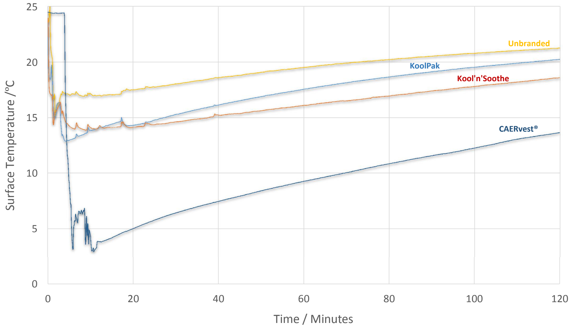
Ambient Temperature Performance (20°C) of CAERvest® Versus Retail Ice Packs
